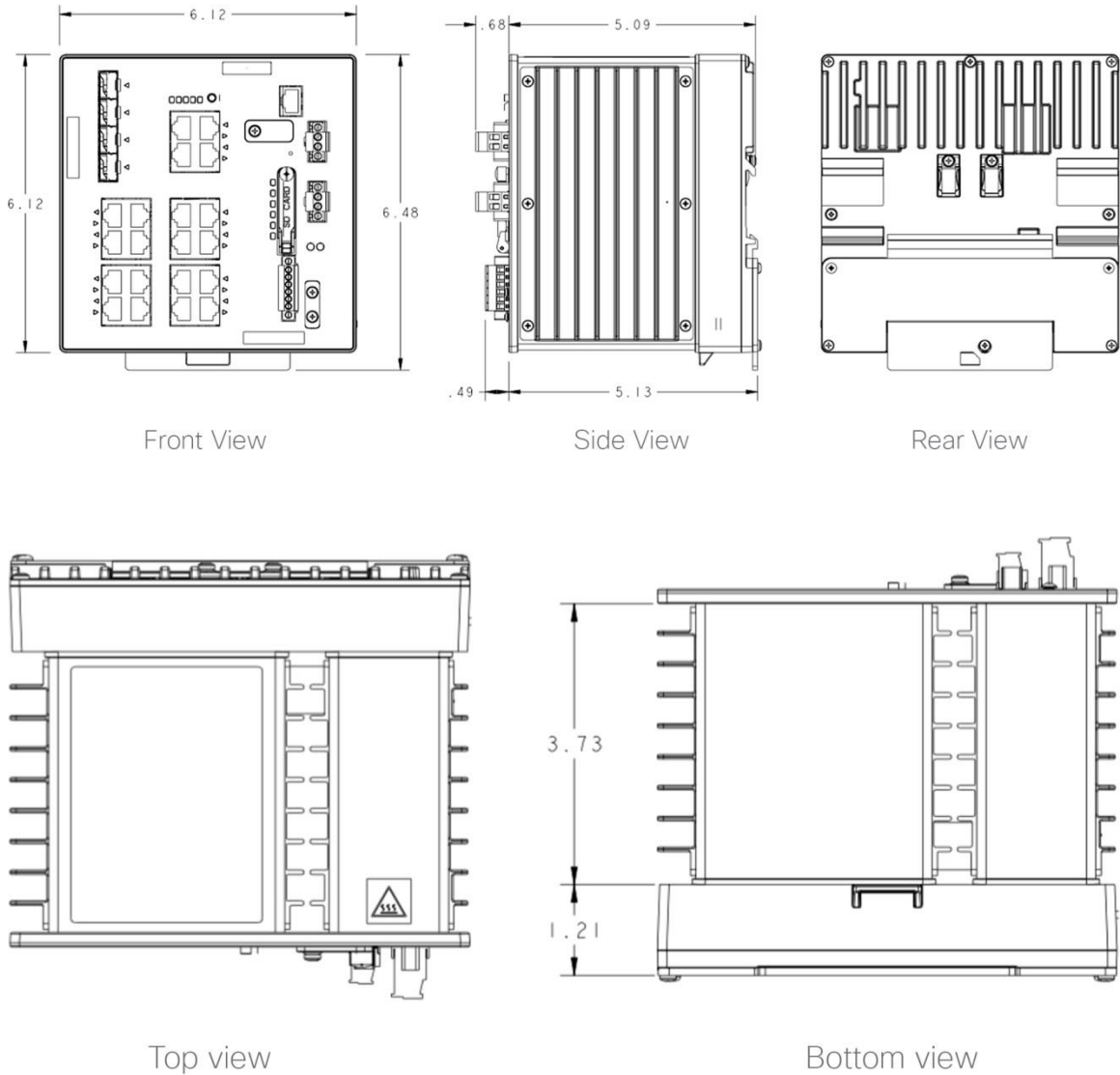
Figure 3. IE-4000 dimensions
